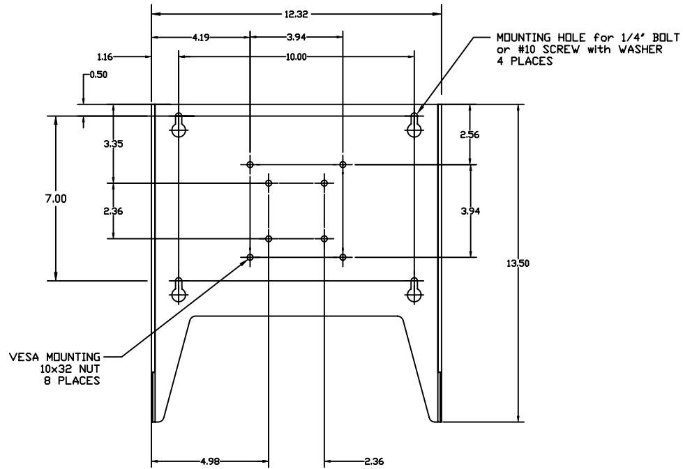
FRONT VIEW (WALL MOUNT BRACKET ONLY)
